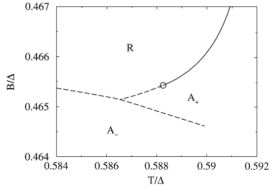
Fig. 10. Detail of a phase diagram in regime 5 ( \Delta = 1.4, \epsilon = 0.01 ). Solid and dashed lines mark second and first order transitions, respectively; circles indicate tricritical points. There is a three-phase point where the three first order lines meet.
