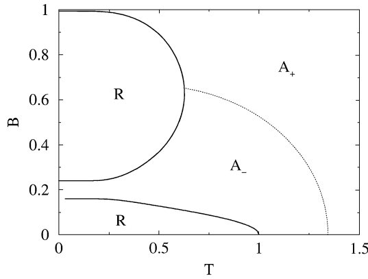
Fig. 8. Phase diagram in regime 2 ( \Delta_{re} < \Delta < 1 ), for \epsilon = 0.4 (where \Delta_{re} = 0.958\dots ) and \Delta = 0.96 . The lines have the same meaning as in Fig. 6. Re-entrant behaviour now occurs even at zero temperature.
