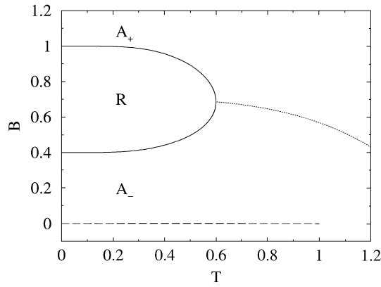
Fig. 3. Phase diagram for the Heisenberg case \Delta = 1 , for \epsilon = 0.4 .
