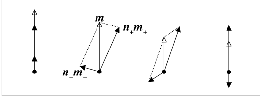
Fig. 2. Geometry of the magnetizations for the Heisenberg model. Shown are (in the xy -plane) the total magnetization \mathbf{m} = n_+\mathbf{m}_+ + n_-\mathbf{m}_- and the sublattice magnetizations scaled by the fractions of spins in the two sublattices, n_+\mathbf{m}_+ and n_-\mathbf{m}_- . The moduli of the sublattice magnetizations m_+ = |\mathbf{m}_+| and m_- = |\mathbf{m}_-| are kept constant while m = |\mathbf{m}| is decreased from left to right. For the maximum value of m , we have an A_+ phase (left), then we obtain an R phase, with \mathbf{m}_- rotating from the positive (upward) towards the negative (downward) z -axis. Finally, when m assumes its minimal value (right), we obtain an A_- phase. This kind of sequence is observed when passing through the R phase in the Heisenberg phase diagram by decreasing the field B at constant T ; the moduli of the sublattice magnetizations remain constant, and they rotate in such a way as to keep \mathbf{m} pointing along the direction of the field (the z -direction).
