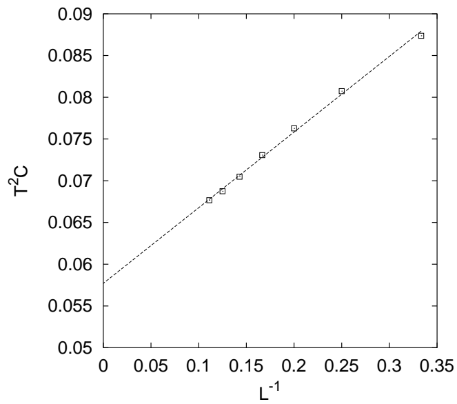
Figure 3. Extrapolation of T^2C near the multicritical point for the three-state Potts model, p = 0.0795 .
